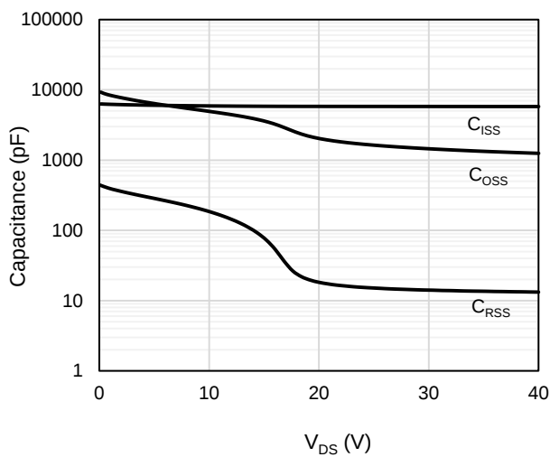
Figure 9: Capacitance Characteristics
