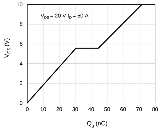
Figure 10: Gate-Charge Characteristics
