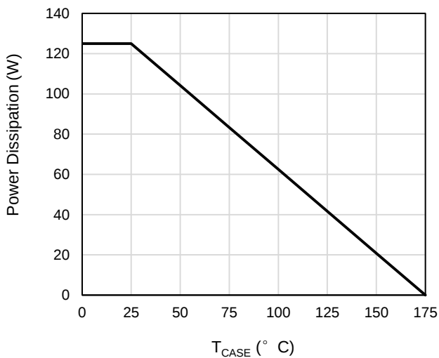
Figure 11: Power De-rating
